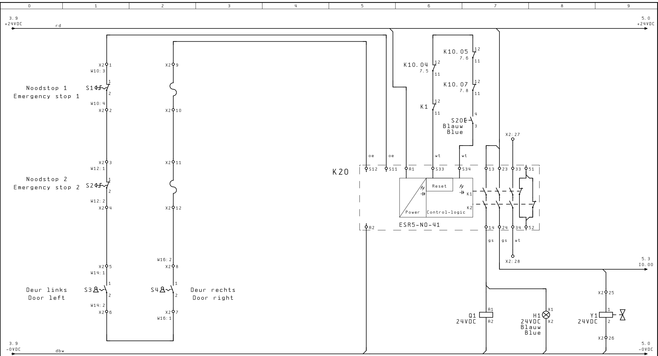
Noodstopcircuit Emergency stop circuit
