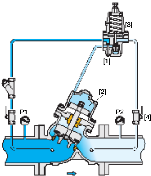
Model 820-PB Apply when P1/P2 > 2.5
